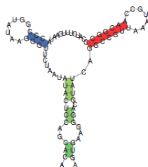
Figure 10.2: The typical representation in textbooks. It clearly shows the secondary substructure in RNA.
