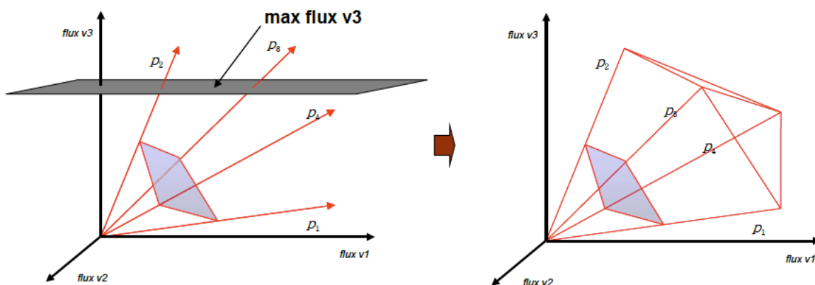
Figure 20.2: Adding constraints to extreme pathways.
