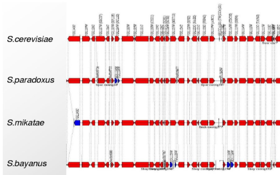
Figure 5.3: Illustration of gene correspondence for S. cerevisiae Chromosome VI (250-300bp).
