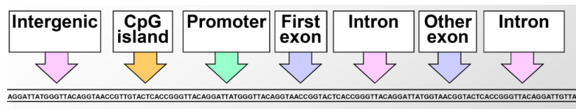
Figure 7.1: Modeling biological sequences
