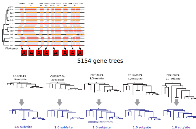
Figure 22.11: We can develop a model for what kind of branch lengths we can expect. We can use conserved gene order to tell orthologs and build trees.
