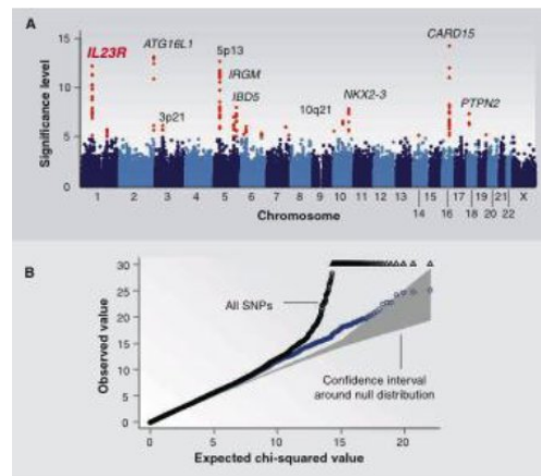
Figure 25.7: (A) Manhattan plot and (B) Q-Q plot for GWAS of Crohn's disease
