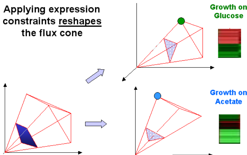
Figure 20.8: Applying expression data set allows constraining of cone shape.
