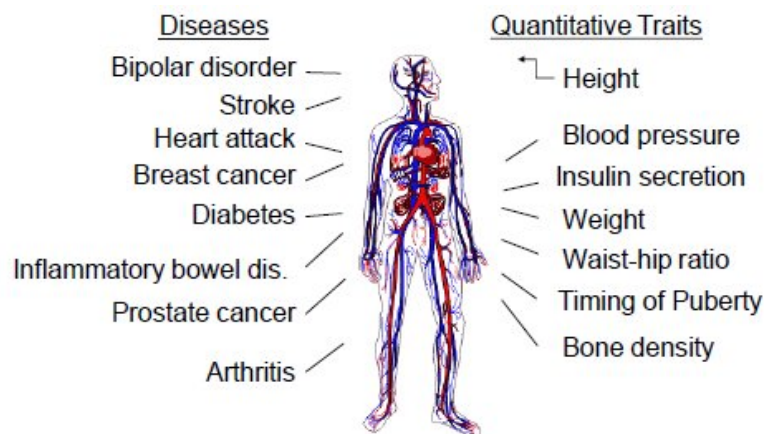
Figure 25.1: Examples of diseases and quantitative traits which have genetic components
