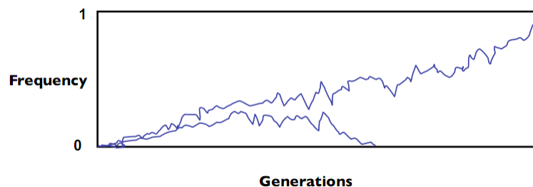
Figure 24.1: Changes in allele frequency over time
