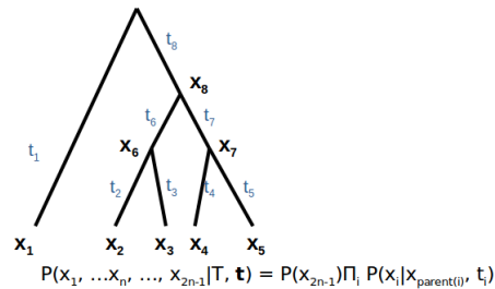
Figure 22.5: Sequence evolution over an entire tree.
