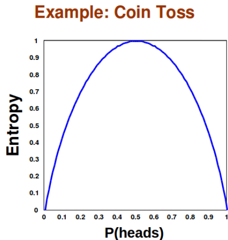
Figure 16.8: Entropy is maximized when the coin is fair, when the toss is most random
