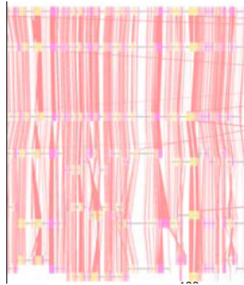
Figure 4.1: Comparative identification of functional elements in 12 Drosophila species
