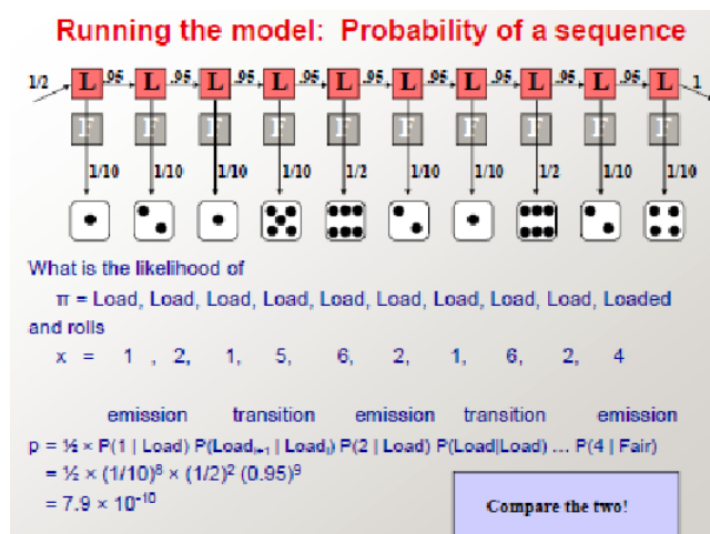
Figure 7.6: Running the model: probability of a sequence (II)
