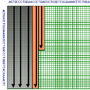
Figure 3.7: Linear-space computation
