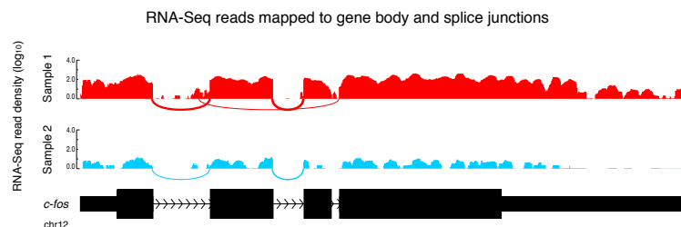
Figure 14.1: RNA-Seq reads mapping to a gene ( c-fos ) and its splice junctions. Densities along exon represent read densities mapping to exons (in \log_{10} ), arcs correspond to junction reads, where arc width is drawn in proportion to number of reads in that junction. The gene is downregulated in Sample 2 compared to Sample 1.
