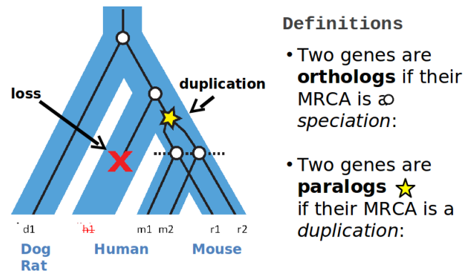
Figure 22.7: Gene Family Evolution: Gene Trees and Species Trees
