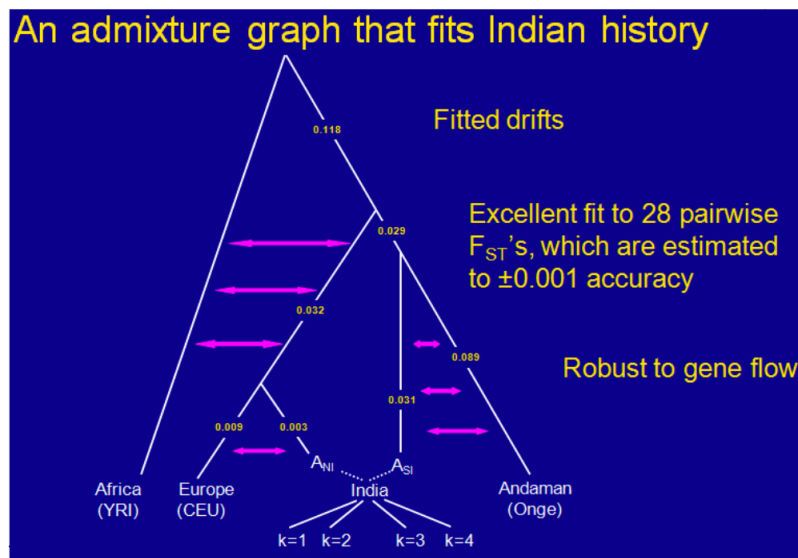
Figure 23.3: An admixture graph that fits Indian history
