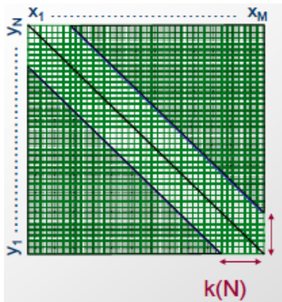
Figure 2.8: Bounded dynamic programming example
