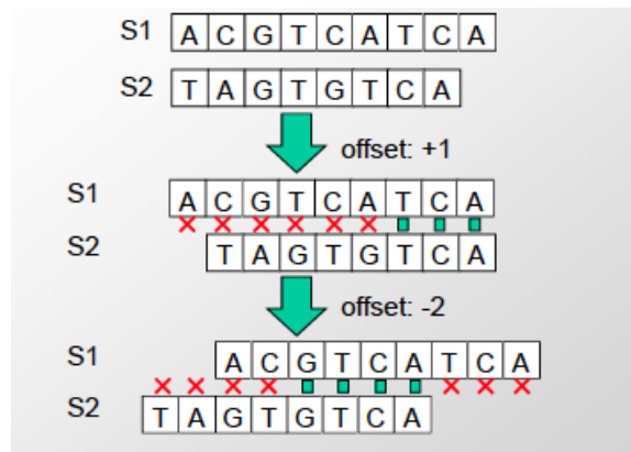
Figure 2.3: Example of longest common substring formulation
