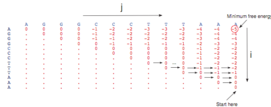
Figure 10.8: The recursion formula for Nussinov algorithm, along with a graphical depiction of how it works.
