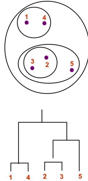
Figure 21.12: UPGMA / Hierarchical Clustering
