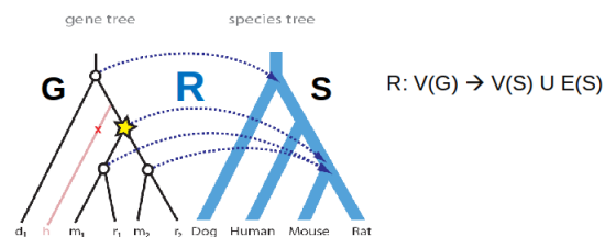
Figure 22.8: Maximum Parsimony Reconciliation (MPR)
