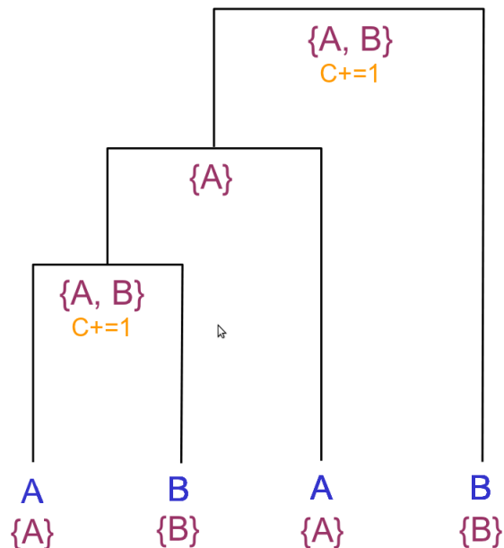
Figure 21.15: Parsimony scoring: union and intersection
