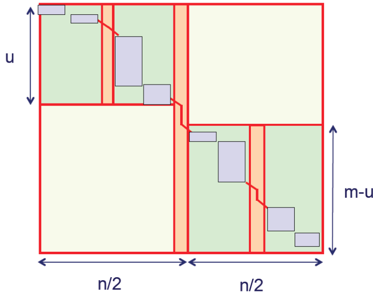
Figure 2.9: Recovering the sequence alignment with O(m + n) space
