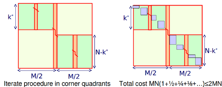
Figure 3.9: Divide and Conquer
