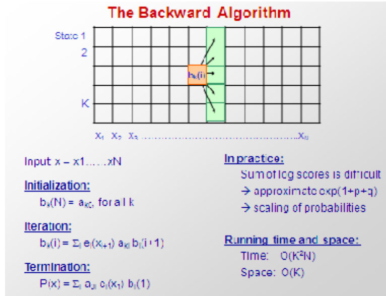
Figure 8.2: The Backward Algorithm
