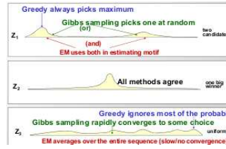
Figure 16.4: Selecting motif location: the greedy algorithm will always pick the most probable location for the motif. The EM algorithm will take an average while Gibbs Sampling will actually use the probability distribution given by Z to sample a motif in each step
