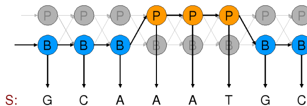
Figure 7.10: HMMS as a generative model
