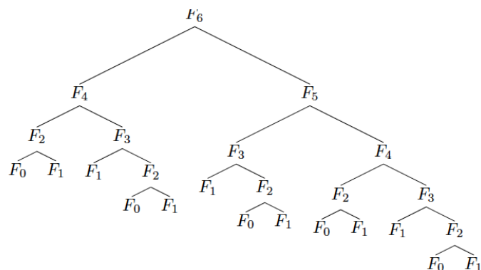
Figure 2.7: The recursion tree for the fib procedure showing repeated subproblems. The size of the tree is O(\phi^n) , where \phi is the golden ratio.
