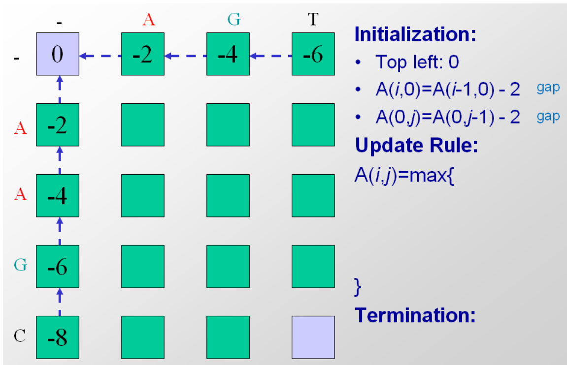
Figure 2.10: (Example) Initial setup for Needleman-Wunsch
