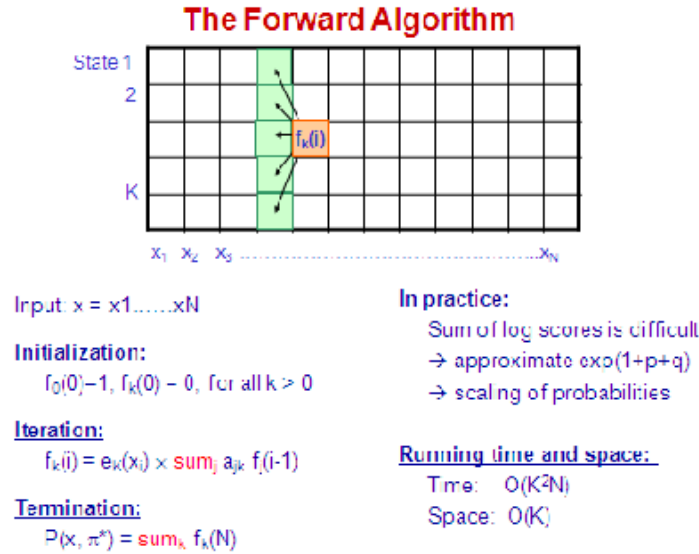
Figure 8.1: The Forward Algorithm
