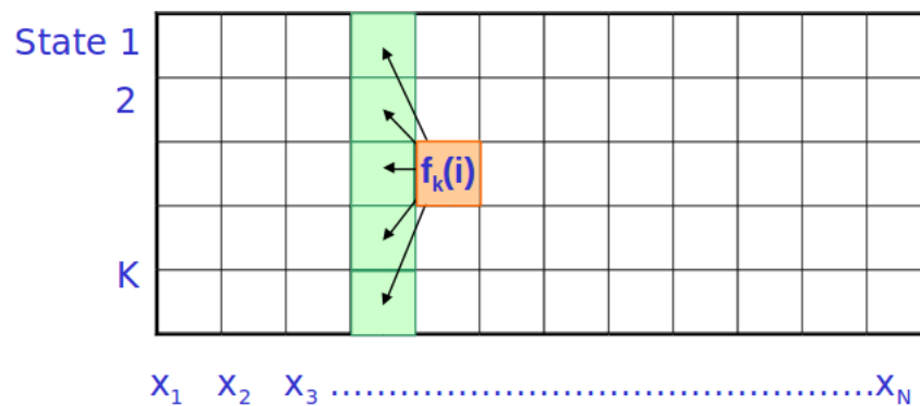
Figure 7.16: The forward algorithm
