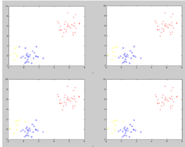
Figure 14.3: From top left moving right, an example of first four iterations of k-means clustering assignments and centroid movements with k=3 . Note the spread of yellow cluster and slight movements of blue and red centroids.
