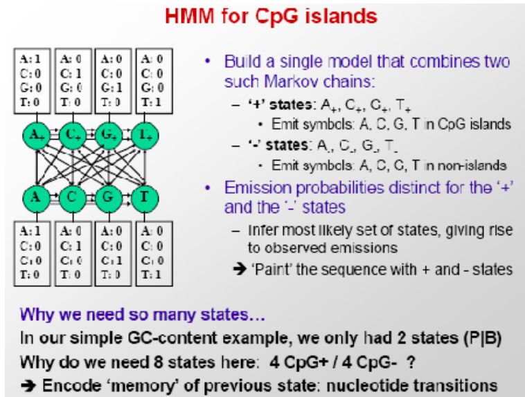
Figure 8.3: HMM for CpG Islands
