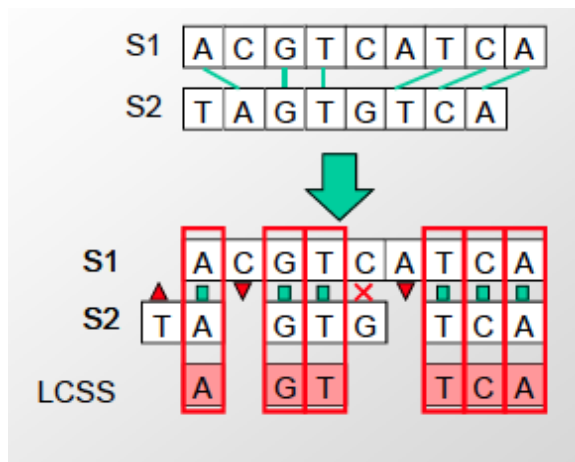
Figure 2.4: Example of longest common subsequence formulation
