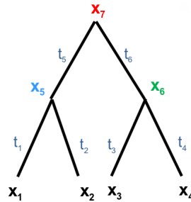
Figure 21.18: A tree to be scored using the peeling algorithm. n=4
