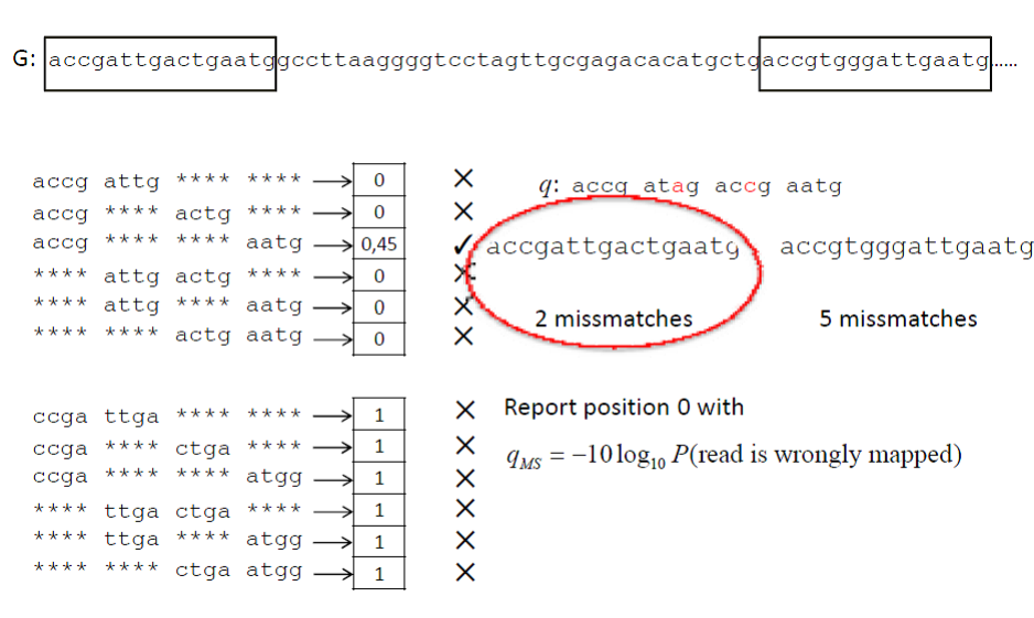
Figure 13.2: Figure 2: Spaced k-mer method of mapping reads to reference genome
