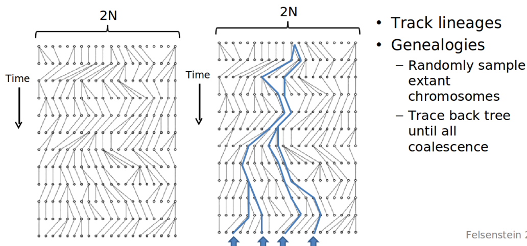
Figure 22.14: The Wright-Fisher model continued over many generations and ignoring the ordering of chromosomes.
