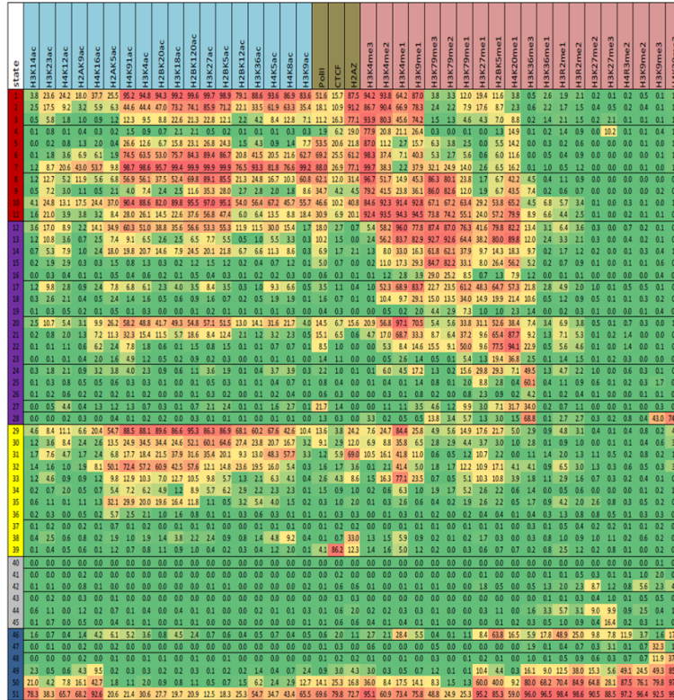
Figure 18.7: Emission probabilities for the final model with 51 states
