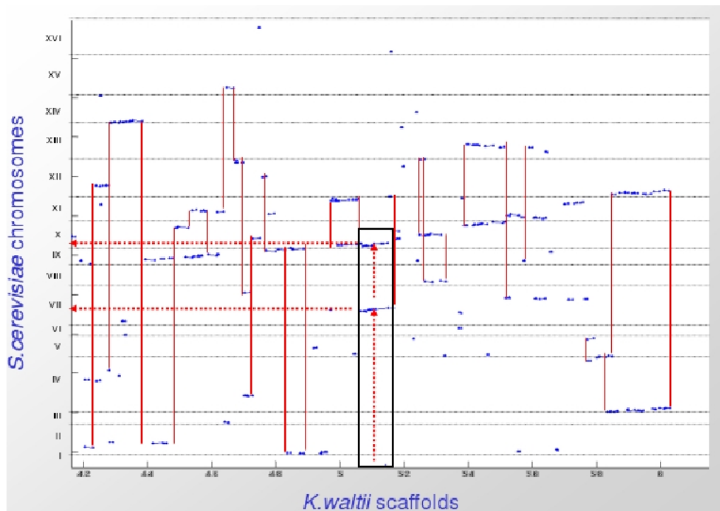
Figure 5.7: Gene Correspondence for S. cerevisiae chromosomes and K. waltii scaffolds.
