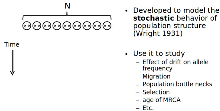
Figure 22.13: The Wright-Fisher model
