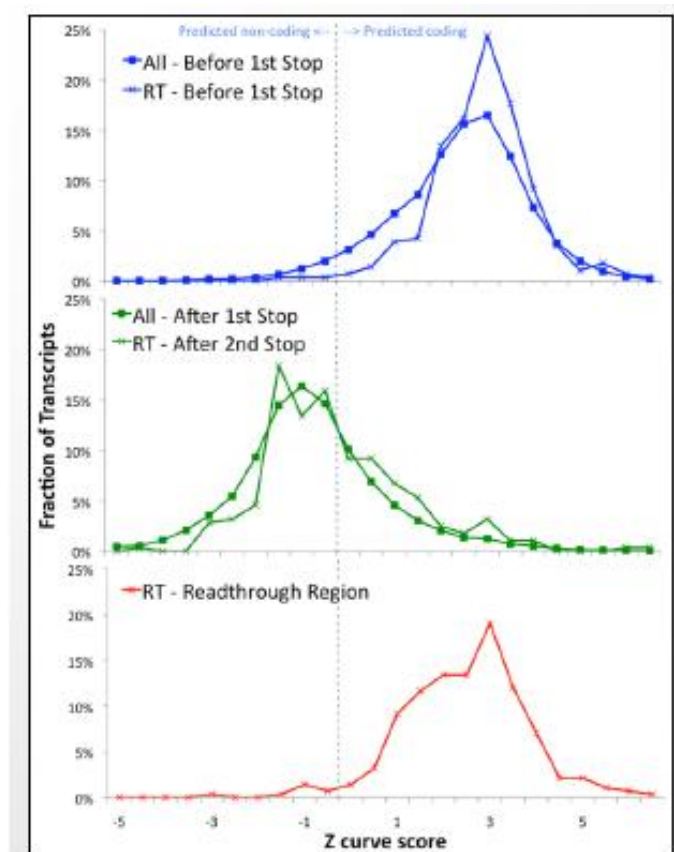
Figure 4.15: Z-curve for Caki . Note that the codon usage in the read through region is similar to that in the region before the first stop codon.
