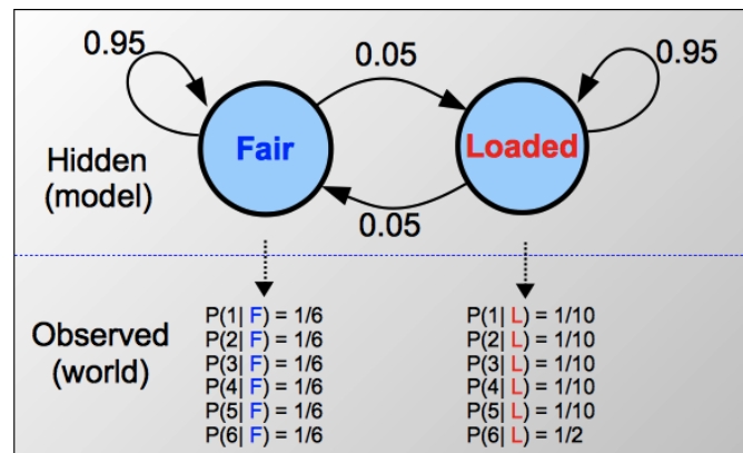
Figure 7.3: State of a casino die represented by a hidden Markov model
