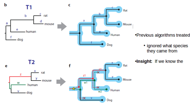
Figure 22.10: Using species trees to improve gene tree reconstruction.
