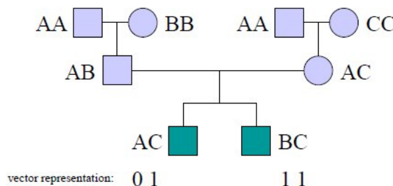
Figure 25.4: Representing a particular pattern of inheritance as an inheritance vector
