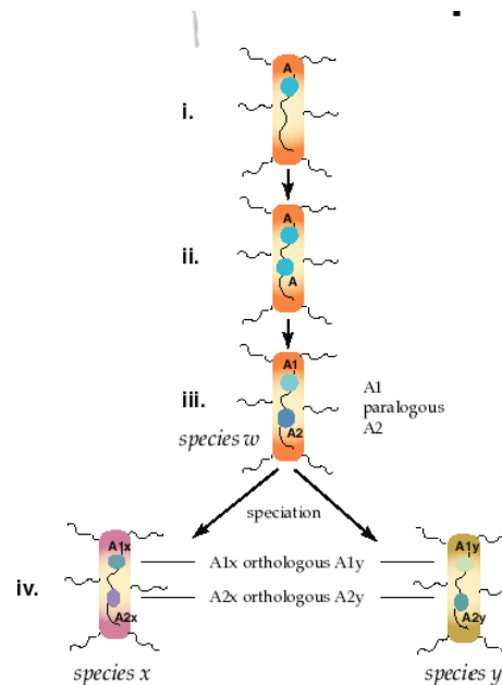
Figure 2.13: Ortholog and paralog sequences
