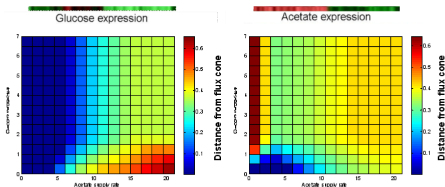
Figure 20.9: Results of nutrient source prediction experiment.
