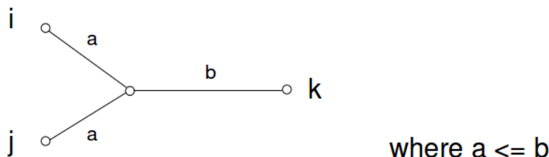
Figure 21.10: Ultrametric distances.
