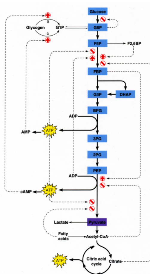
Figure 20.1: The process leading to and including the citric acid cycle.
