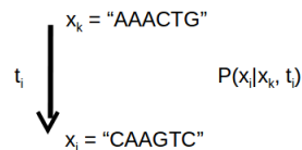
Figure 22.4: Sequence evolution is the product of site evolution
