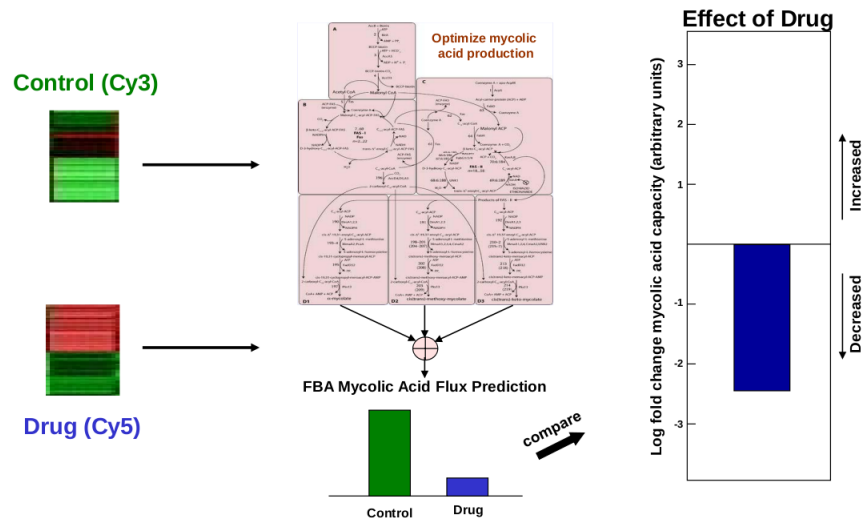
Figure 20.7: Basic flow in predicting state of a metabolic system under varying drug treatments
