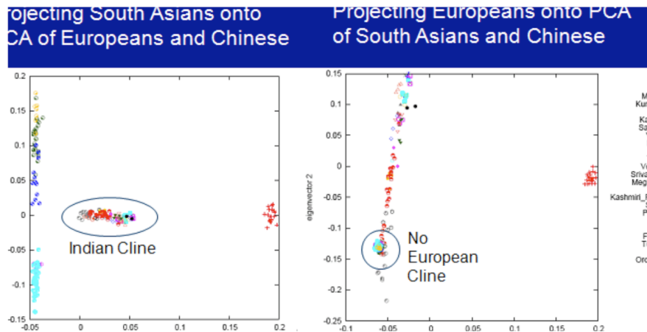
Figure 23.2: Populations can be projected onto the principal components of other populations: South Asians projected onto Chinese and European principal components produces a linear effect (the India Cline), while Europeans projected onto South Asian and Chinese principal components does not.
