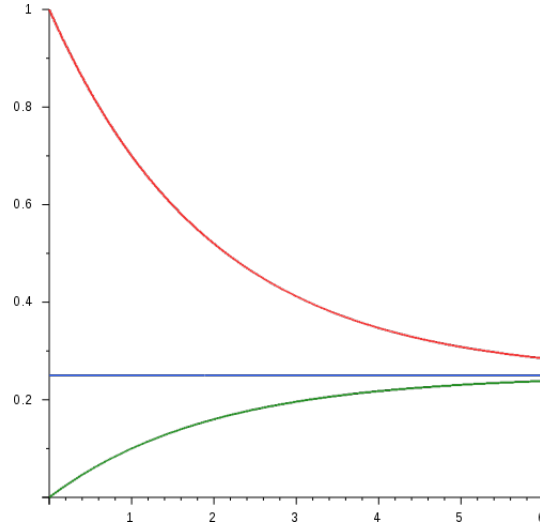
Figure 21.6: The y axis denotes probability of observing the bases - A(red), others(green). x axis denotes time.
