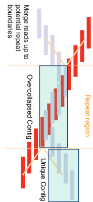
Figure 5.9: Merging reads.
