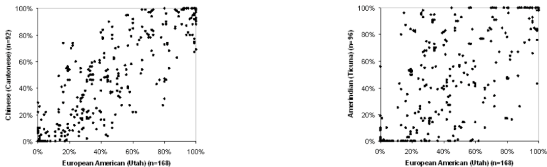
Figure 23.1: Similarity between two subpopulations can be measured by comparing allele frequencies in a scatterplot. The plots show the relative dissimilarity of European American and American Indian populations along with greater similarity of European American and Chinese populations.
