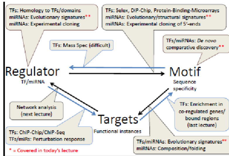
Figure 17.1: Challenges in Regulatory Genomics
