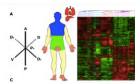
Figure 11.1: Human fibroblasts specialize via epigenetic regulation to form different skin types based on their location within the body. Research has found that the type of skin in the hands shares a remarkably similar epigenetic signature to the skin in the feet, which is also distally located.
