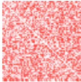
Figure 4.7: Rate matrix Q_N estimated from non-coding regions
