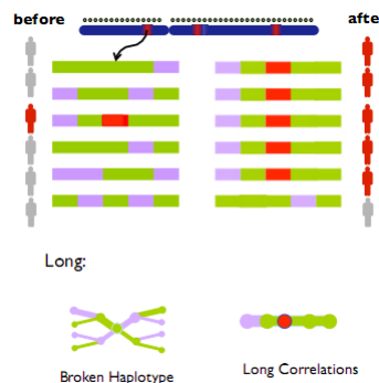
Figure 24.3: Genomic Signals of Natural Selection
