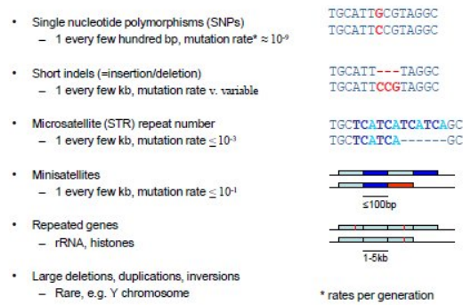
Figure 25.6: Different types of genetic variation
