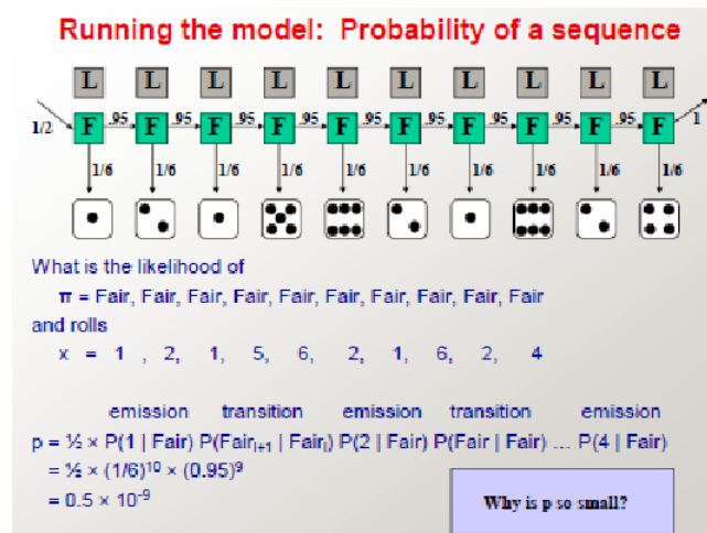
Figure 7.5: Running the model: probability of a sequence (I)
