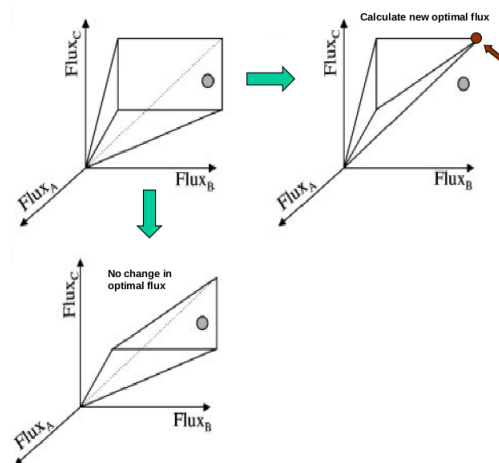
Figure 20.5: Constraining the feasible solution space may create a new optimal flux.
