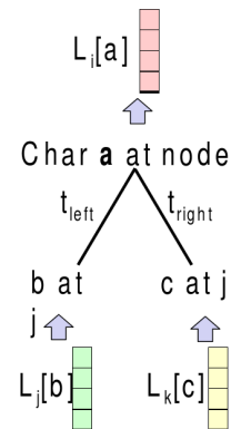
Figure 19: The recursive algorithm for computing the probability of a tree.
