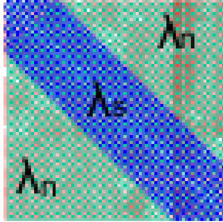
Figure 4.18: We can measure \lambda_s and \lambda_n , which give the rate of synonymous and nonsynonymous substitutions, respectively, in a given region.
