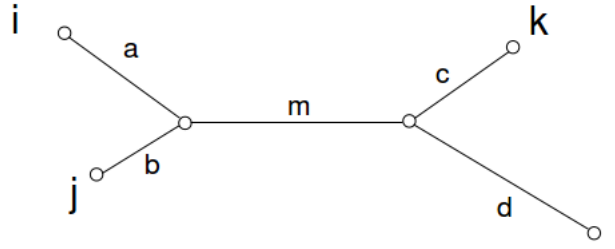
Figure 21.11: Additive distances.
