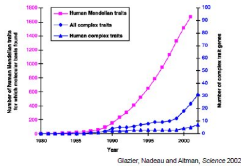
Figure 25.5: Discovery of genes for different disease types versus time
