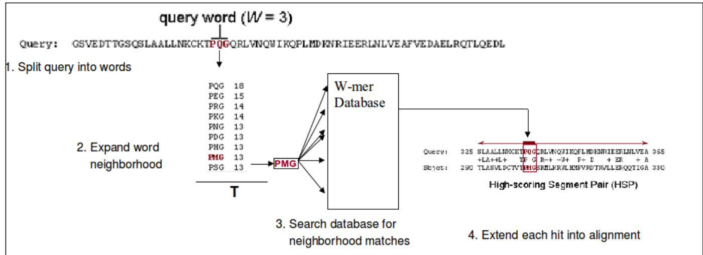
Figure 3.13: The BLAST Algorithm
