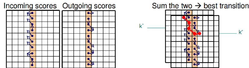
Figure 3.8: Space-saving optimization
