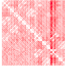
Figure 4.6: Rate matrix Q_C estimated from known coding regions
