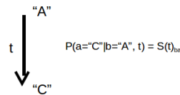
Figure 22.3: Site evolution uses the Jukes-Cantor model
