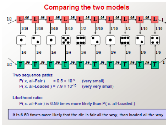
Figure 7.7: Comparing the two models
