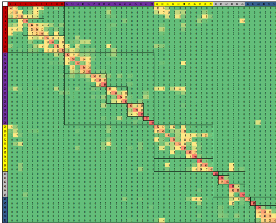
Figure 18.8: Transition probabilities for the final model with 51 states
