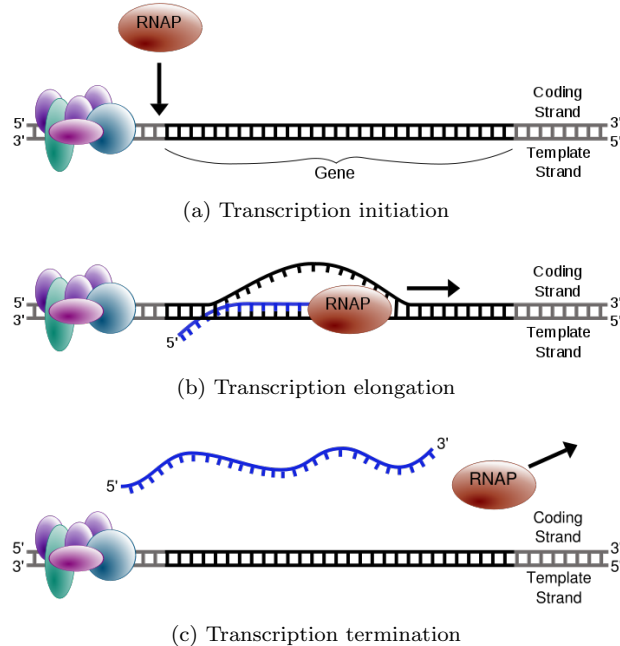
Figure 1.4: RNA is produced from a DNA template during transcription. A bubble is opened in the DNA, allowing the RNA polymerase to enter and place down bases complementary to the DNA.
