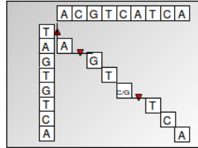
Figure 3.1: Global Alignment
