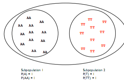
Figure 24.2: Two isolated populations
