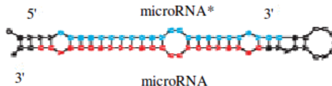
Figure 4.9: The hairpin structure of a microRNA. Note that microRNA* denotes the strand on the opposite side of the hairpin that is expressed at lower levels (ref).
