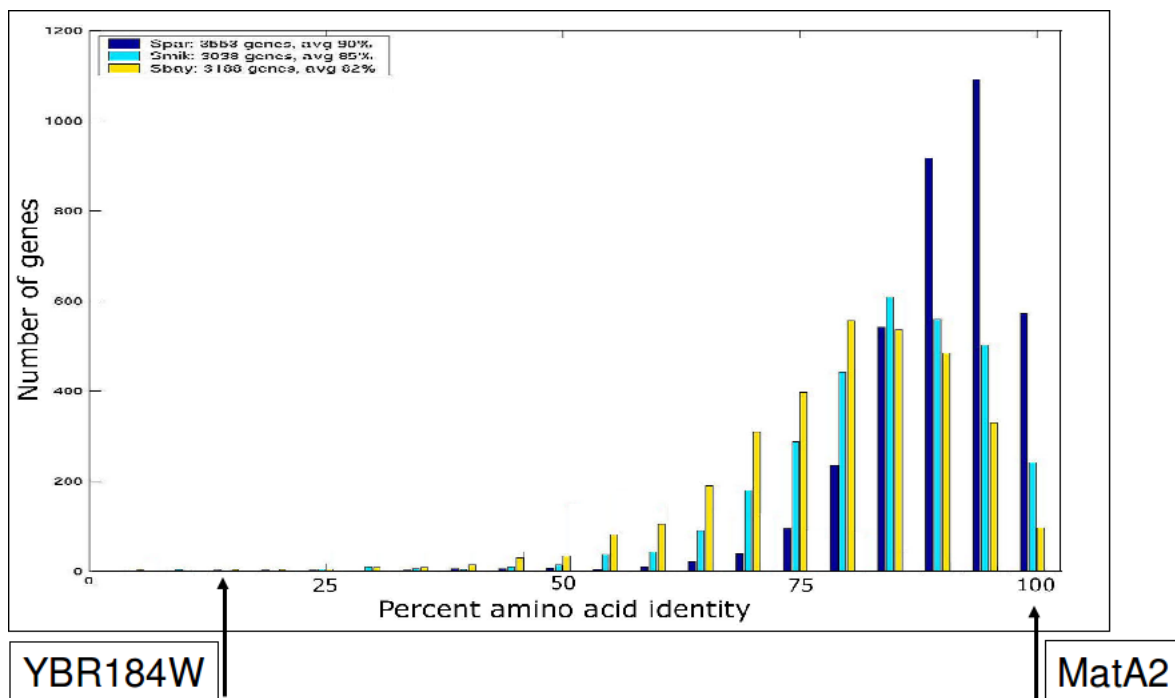
Figure 5.4: Dynamic view of a changing gene
