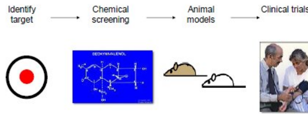
Figure 25.2: The drug development process
