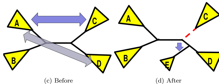
Figure 21.20: An unit step using Nearest Neighbor Interchange scheme
