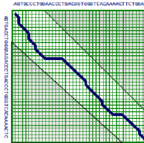
Figure 3.6: Bounded-space computation
