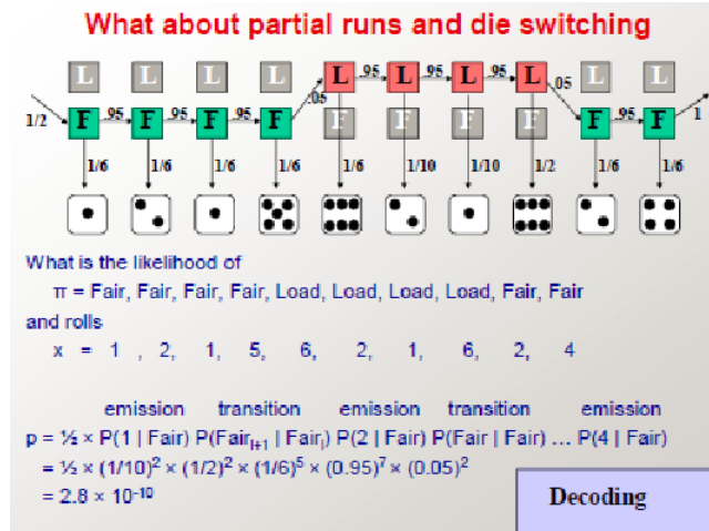
Figure 7.8: Partial runs and die switching
