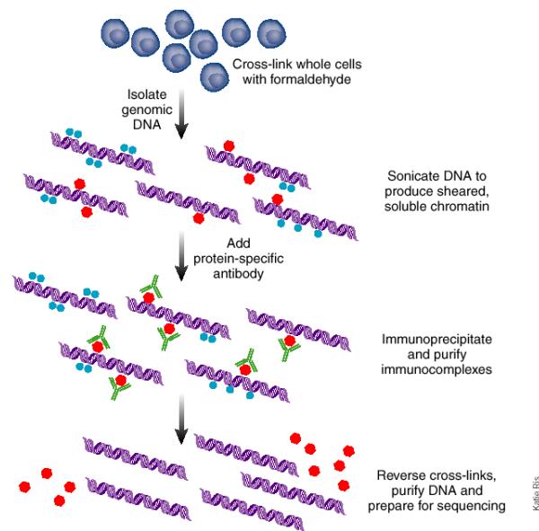
Figure 18.2: Chromatin immunoprecipitation [4]
