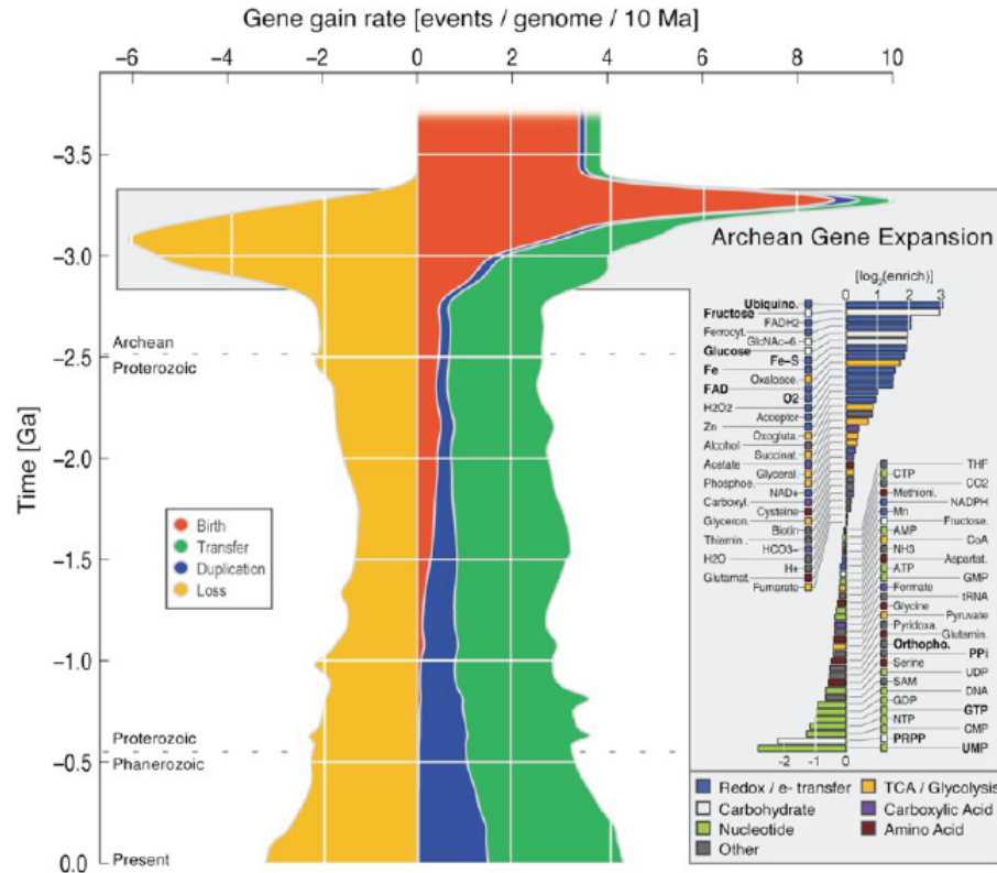
Figure 6.2: Rates of new gene birth, duplication, loss and horizontal gene transfer during Archean Gene Expansion
