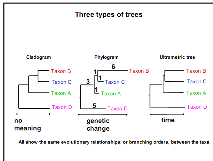
Figure 21.3: Three types of trees.
