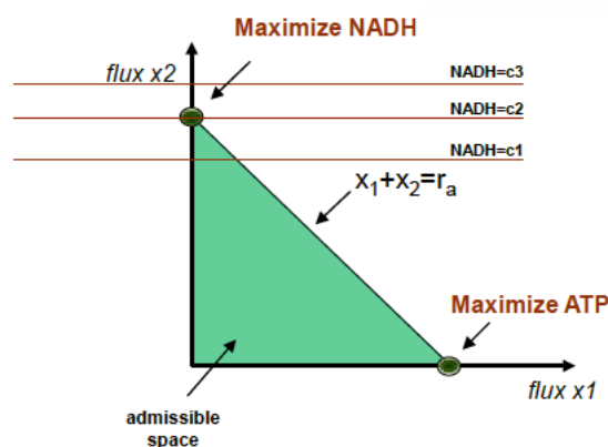
Figure 20.3: Maximizing two functions with linear programming.
