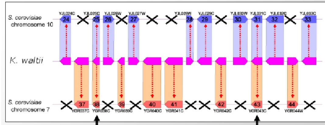
Figure 5.8: Gene interleaving shown by sister regions in K.waltii and S.cerevisiae
