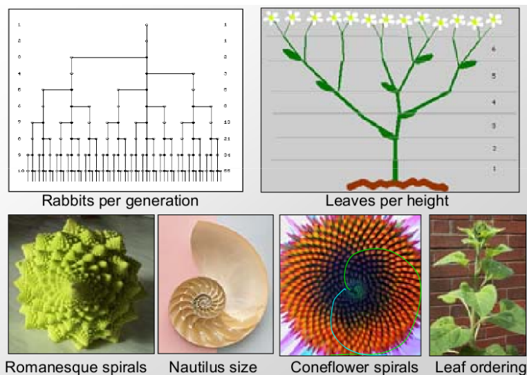
Figure 2.6: Examples of Fibonacci numbers in nature are ubiquitous.
