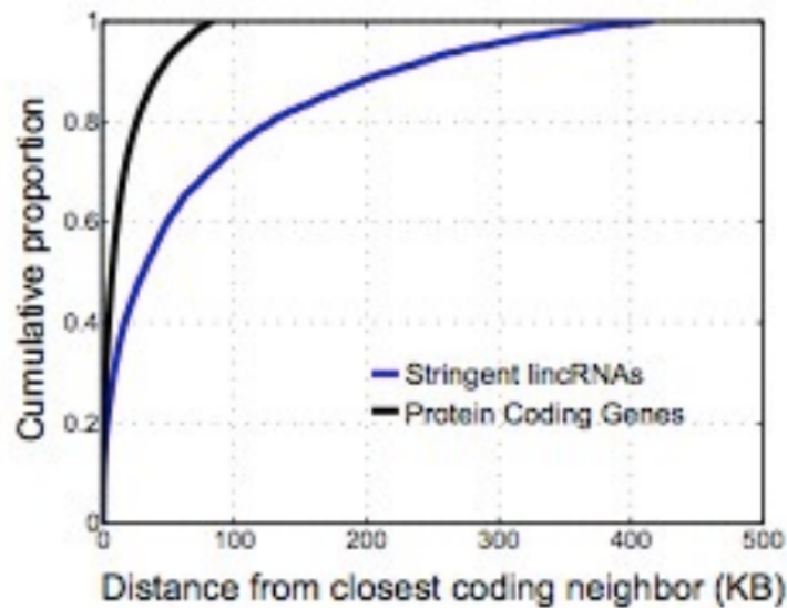
Figure 11.4: lincRNAs neighbor developmental regulators
