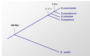
Figure 5.6: Moving further back in evolutionary time for Saccharomyces .
