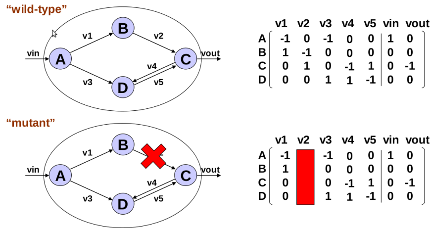
Figure 20.4: Removing a reaction is the same as removing a gene from the stoichiometric matrix.
