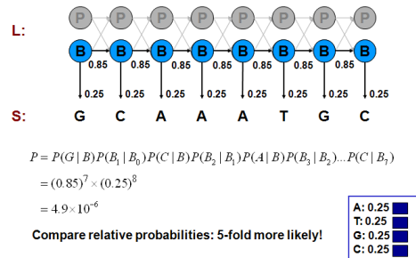
Figure 7.12: Probability of seq, path if all background
