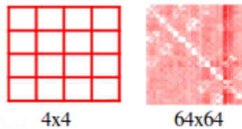
Figure 4.17: We can represent the null model, which contains regions without excess constraint, as a rate matrix. If we are looking at the nucleotide level, we can use a 4x4 matrix to model substitution rates between nucleotides. If we are looking at codons, we can use a 64 by 64 matrix to model substitution rates between codons.
