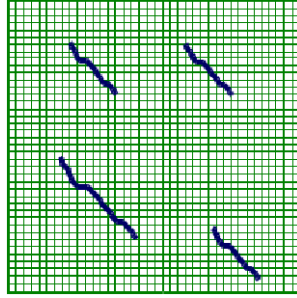
Figure 3.3: Local Alignment
