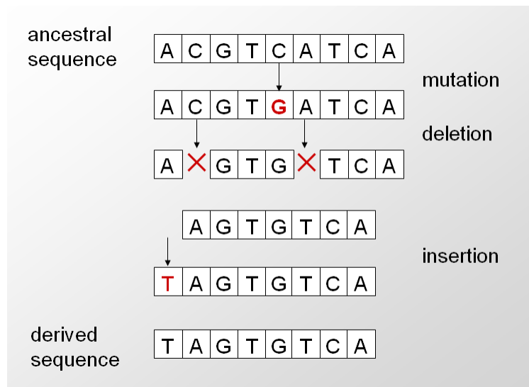
Figure 2.2: Evolutionary changes of a genetic sequence
