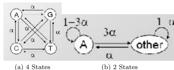
Figure 21.5: Markov chain accounting for back mutations
