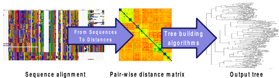
Figure 21.4: The two steps of distance based phylogenetic reconstruction.
