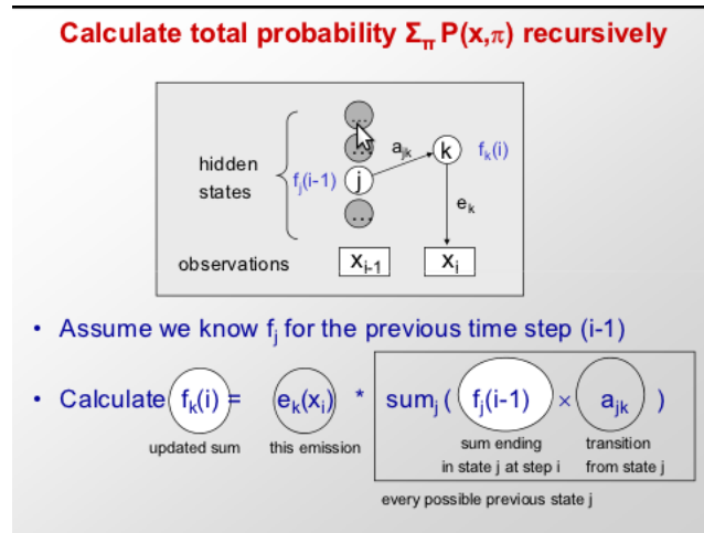
Figure 7.15: Calculate total probability recursively
