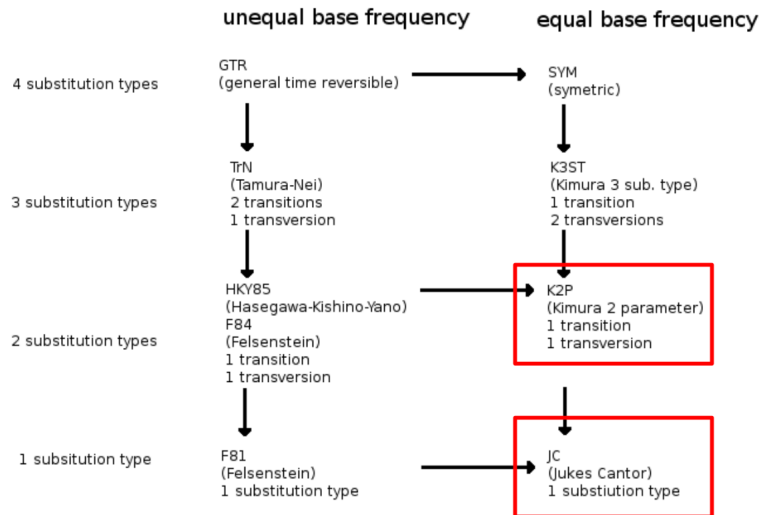
Figure 21.8: Distance models of varying levels of complexity(parameters).
