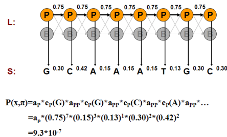
Figure 7.11: Probability of seq, path if all promoter
