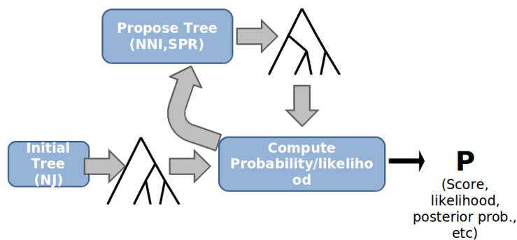
Figure 21.14: An overview of the character based methods
