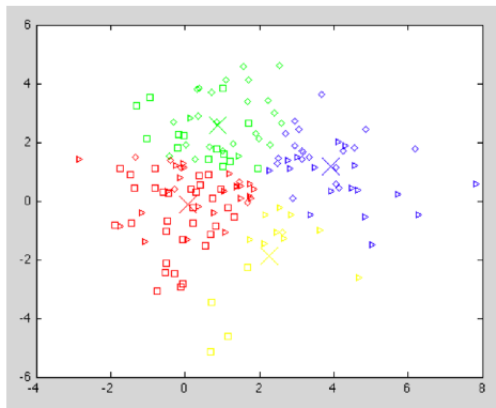
Figure 14.4: Examples of final cluster assignments of fuzzy k -means using k=4 with centroids, correct clusters, and most probable assigned clusters marked as crosses, shapes shapes of points, and colors respectively. Note that the original data set is non-Gaussian.
