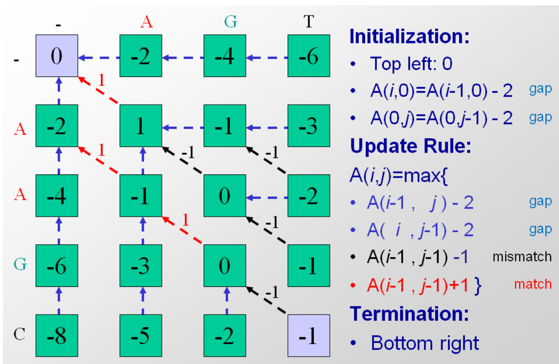
Figure 2.11: (Example) Half-way through the second step of Needleman-Wunsch
