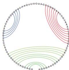
Figure 10.3: As a graph drawing the back-bone as a circle and the base pairing as arcs within the circle. Note that the graph is outer-planar, meaning the arcs do not cross.
