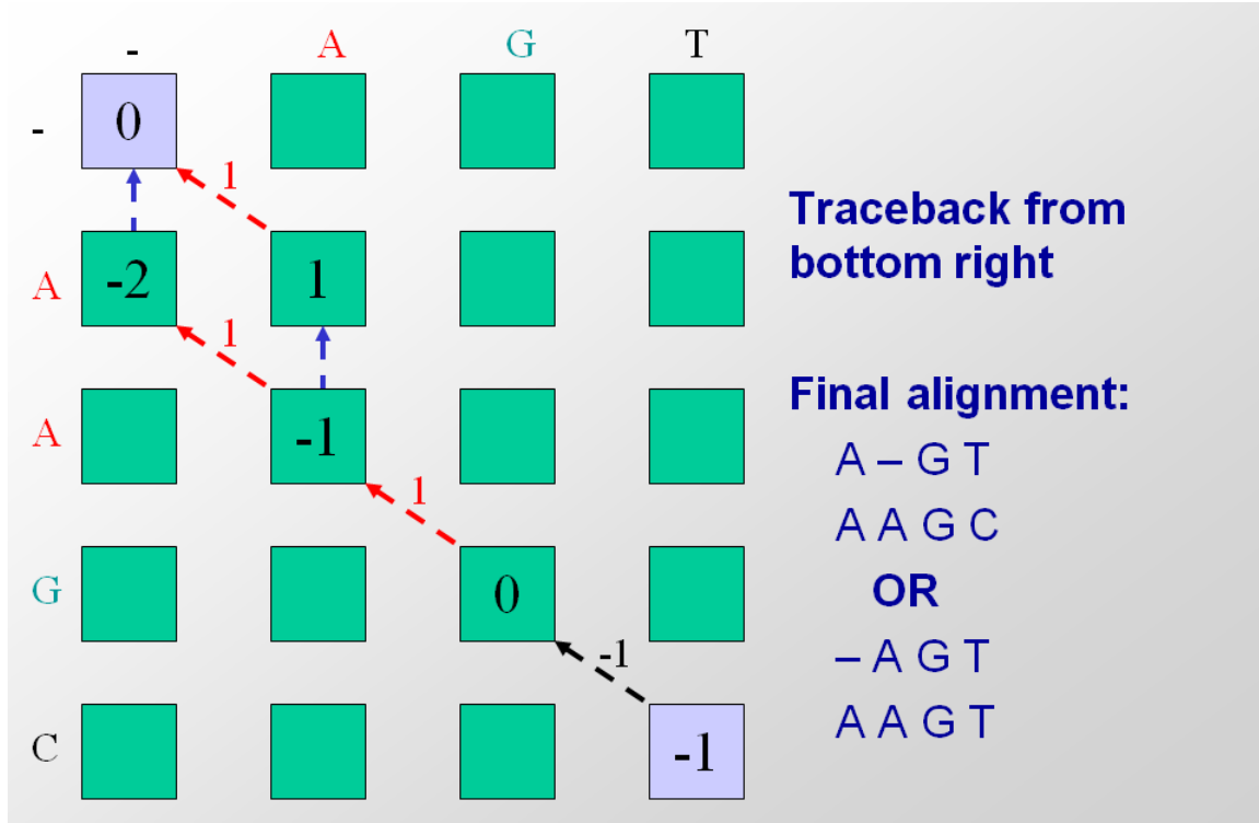
Figure 2.12: (Example) Tracing the optimal alignment
