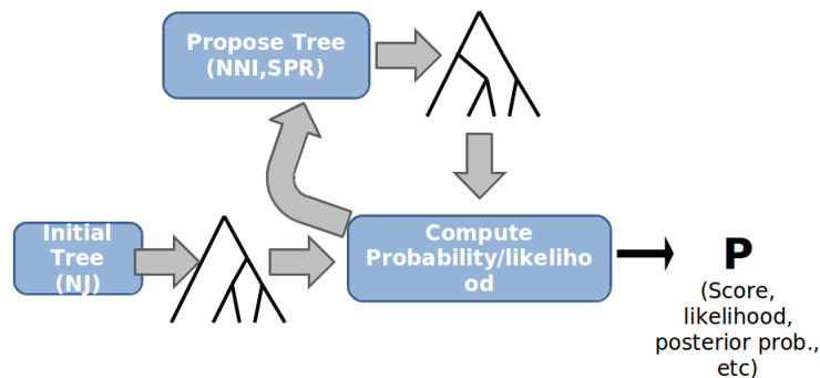
Figure 22.1: Heuristic tree search in character-based reconstruction
