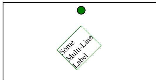
Figure 5-10: Label example
