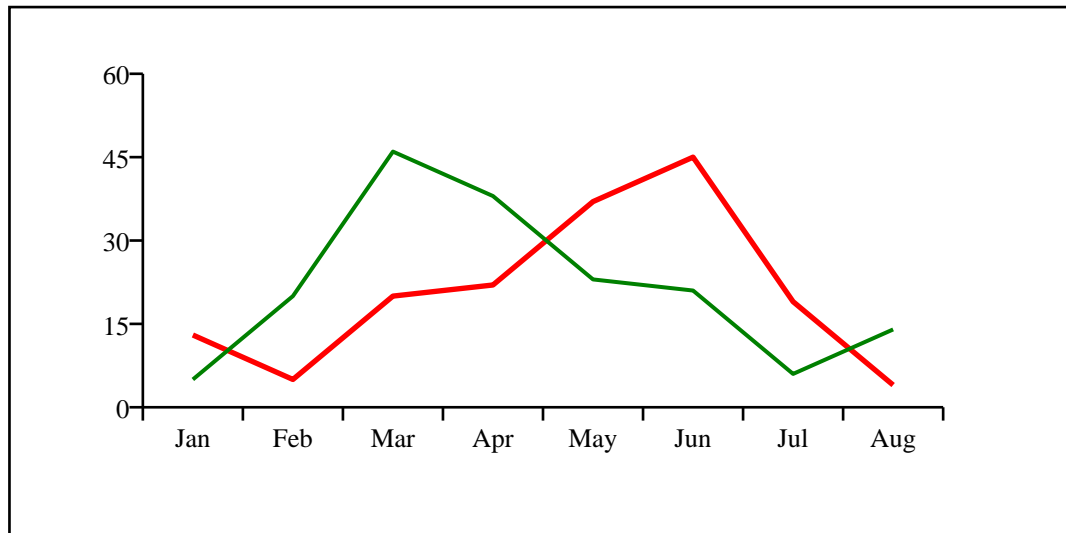
Figure 5-15: HorizontalLineChart sample
