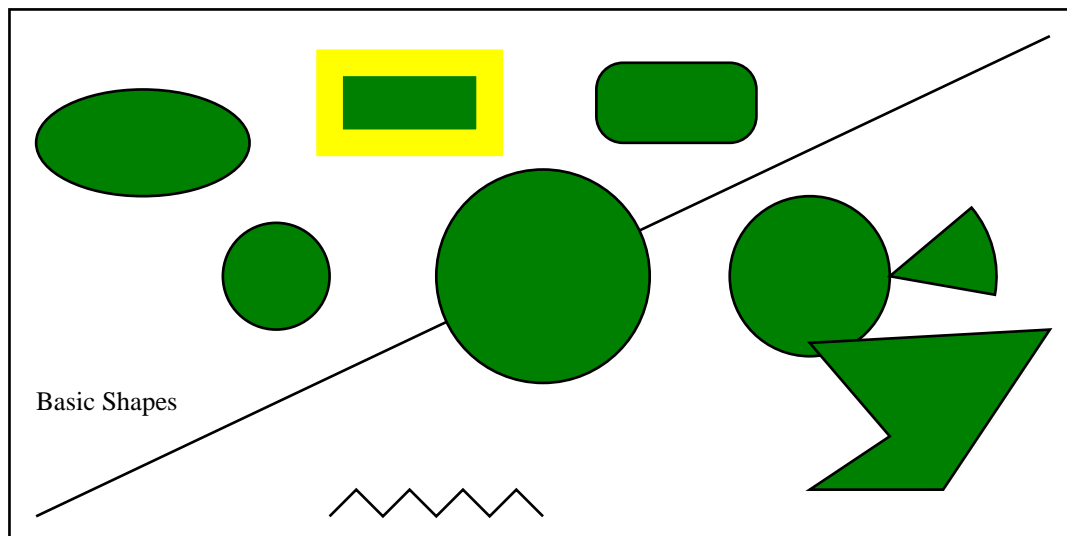
Figure 5-2: Basic shapes
