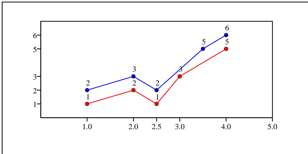
Figure 5-16: LinePlot sample
