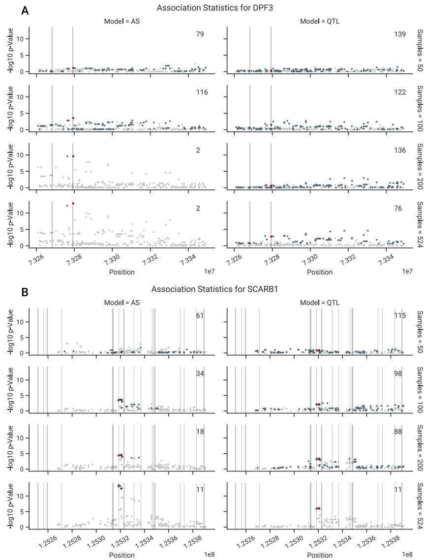
Figure 6: Comparison of AS and QTL associations in the experimentally-verified loci, as a function of sample size. Regions of 70 kb are shown around the causal marker. AS and QTL p-Values were calculated using from z_\phi and z_\beta , respectively. Fine-mapping was conducted with the PLASMA-AS and QTL-Only models, respectively. 95% credible set sizes for the whole locus are displayed in the top right of each subplot. Markers in the 95% credible set are shown in dark gray, while markers not in the sets are shown in light gray. The experimentally verified causal marker is shown in red. Regions of open chromatin (DNase-Seq peaks) are shaded in gray. (a) Associations in the DPF3 locus (b) Associations in the SCARB1 locus.
