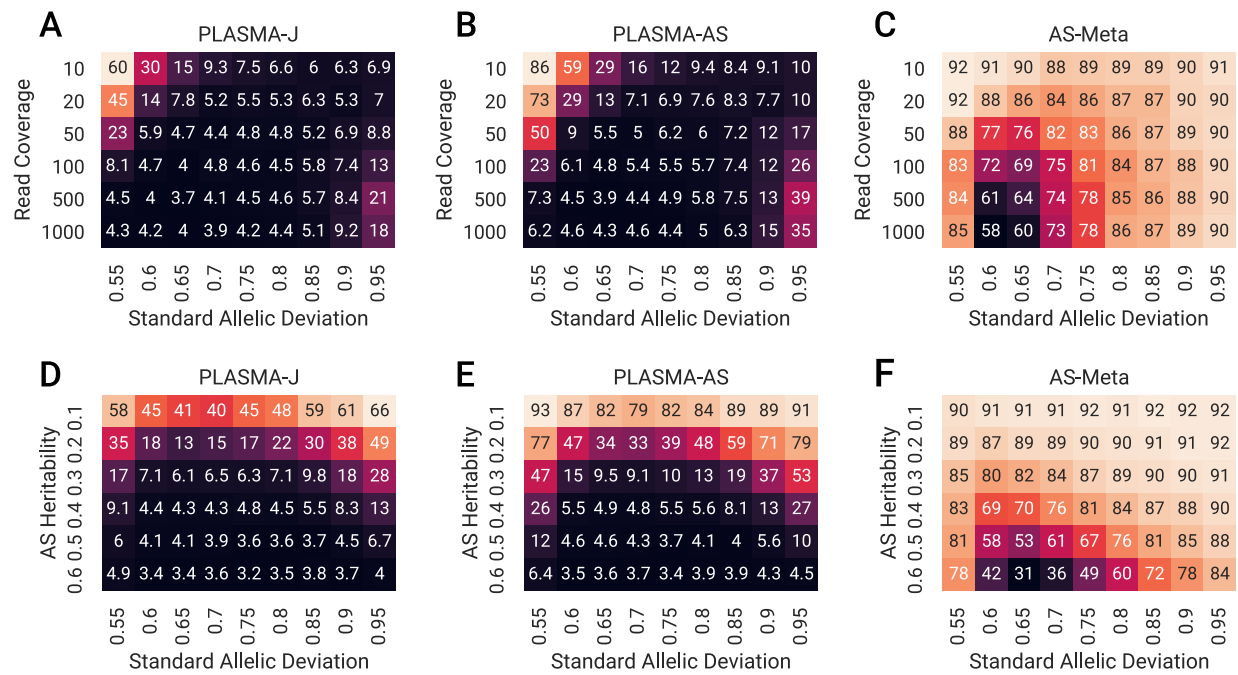
Figure 3: Comparison of the mean 95% confidence credible set sizes across different AS fine-mapping methods. Each square is the mean set size calculated over 500 simulated loci of 100 markers and 100 samples each, with one causal variant. (a, b, c) Mean credible set sizes as a function of standard allelic deviation and mean read coverage, with AS heritability set to 0.4. (d, e, f) Mean credible set sizes as a function of standard allelic deviation and AS heritability, with mean read coverage set to 100 reads.
