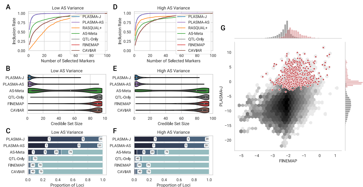
Figure 2: Comparison of fine-mapping methods on two sets of simulated loci of 100 markers and 100 samples each. These two sets differ in the variance of the AS phenotype, but with a fixed mean coverage and AS heritability. (a, d) Inclusion curve at low and high AS variance, respectively (0.6, 0.8 standard allelic deviation). The y-axis shows the expected proportion of markers included in the credible set, and the x-axis shows the number of selected markers by posterior probability. (b, e) Distribution of 95% confidence credible set sizes at low and high AS variance, respectively. (c, f) Proportions of loci with 95% credible set sizes within given thresholds at low and high AS variance, respectively. Thresholds used are 1, 5, 20, 40, 70, and 100 markers. (g) A per-snp fine-mapping comparison between PLASMA-J and FINEMAP across 500 simulated loci with one causal variant each. The axes denote the posterior log-odds of causality for FINEMAP and PLASMA-J, respectively. The black hexagons represent the joint distribution of all markers, while the red dots represent specifically the causal markers. Univariate histograms for PLASMA-J and FINEMAP are plotted along the margins.
