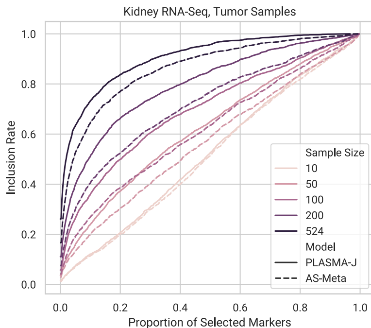
Figure S8: Inclusion curve for fine-mapped kidney tumor RNA-Seq data for PLASMA and AS-Meta across sample sizes. Inclusion was evaluated against a gold-standard set of markers, defined as all markers with at least 0.1 posterior probability under FINEMAP with all samples.
