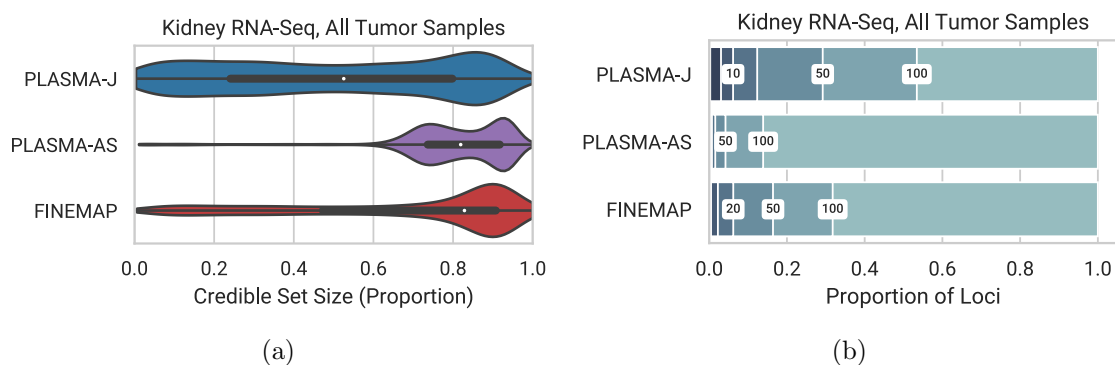
Figure S9: Fine-mapping of kidney RNA-Seq loci under the assumption of up to three causal variants. (Note that FINEMAP credible sets may not be calibrated under multiple causal variants.) (a) 95% confidence credible sets. (b) Proportions of loci with 95% credible set sizes within given thresholds. Thresholds used were 1, 5, 10, 20, 50, and 100.
