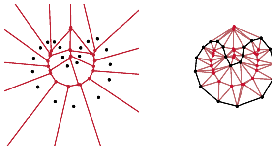
Figure 5. The two-dimensional algorithm. On the left, the Voronoi diagram of a point set S sampled from a curve. Just as S approximates the curve, the Voronoi vertices V approximate the medial axis of the curve. On the right, the the Delaunay triangulation of S \cup V , with the crust edges in black. Theorem 1 states that when S is an r -sample, for sufficiently small r , the crust edges connect only adjacent vertices.
