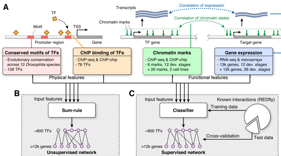
Figure 1. Overview of inference methodology for supervised and unsupervised functional regulatory networks. (A) The four types of input features to the network inference algorithms are: evolutionarily conserved motifs (red) and ChIP-based binding (orange) of TFs near the transcription start site (TSS) of target genes (physical features), and correlation of chromatin (green) and expression (blue) profiles between TFs and target genes (functional features). (B) Unsupervised network inference: An integrative network is formed by adding the evidence from each input feature with equal weight (sum-rule). (C) Supervised network inference: The input features are used in a classifier that predicts for every TF–target pair the presence or absence of a regulatory interaction. The classifier is trained on a literature-curated set of known interactions (REDfly).
