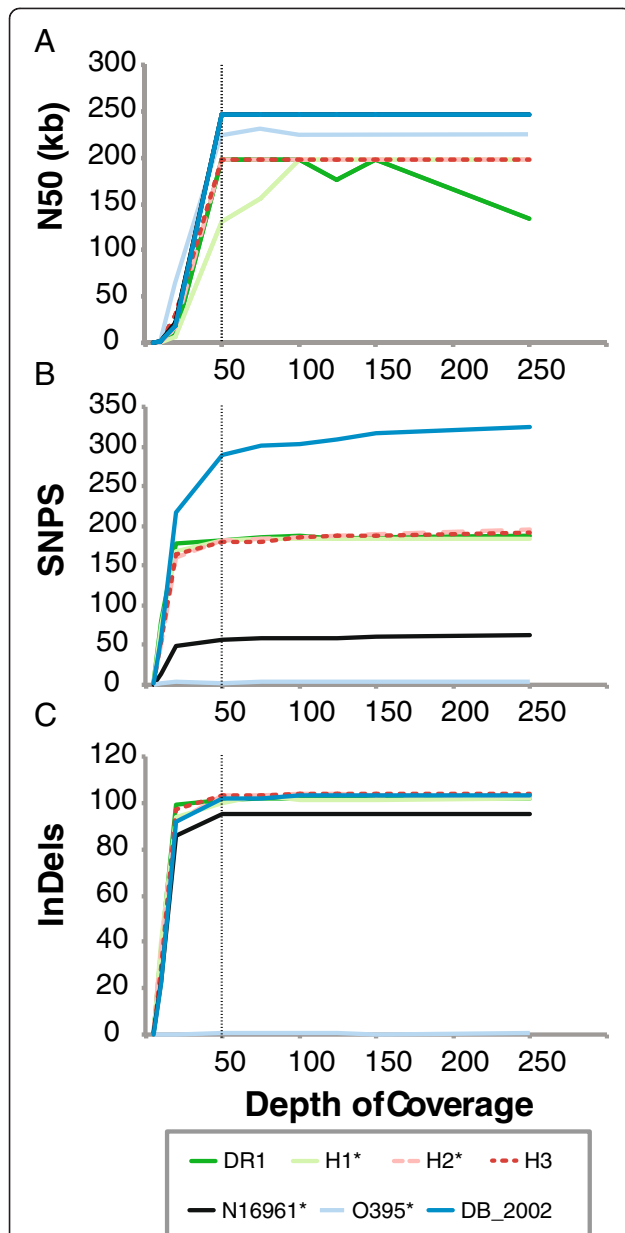
Figure 1 Fiftyfold coverage suffices for whole-genome assembly and detection of most sequence variants. (A) The N50 of the assembly, shown over a range of coverage depths (5x-250x), rapidly increases up to 50x coverage, and then plateaus. The median N50 of assemblies of five disjoint sets of reads at each depth of coverage is shown. (B) The number of SNPs detected increases rapidly up to 50x coverage, and gradually thereafter. (C) The number of insertions and deletions detected increases rapidly up to 20x coverage, and plateaus after 50x coverage. SNPs, insertions, and deletions in all isolates except for O395* are called relative to the N16961 genome [GenBank:AE003852, GenBank:AE003853]. For the O395* sample, due to the large number of differences (>20,000 SNPs) from the N16961 reference, SNPs, insertions, and deletions were identified instead against the Sanger-sequenced O395 reference [GenBank:CP000626, GenBank:CP000627].
